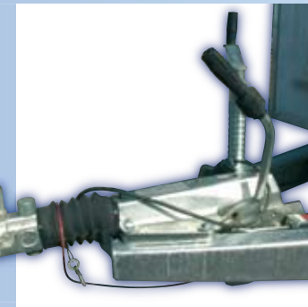
TripleLock – lockable coupling head
